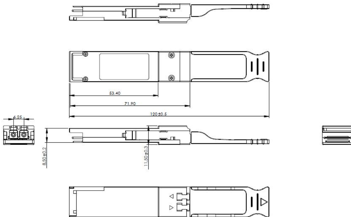
Figure 4. Mechanical Outline
